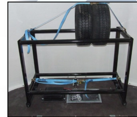
TYRE RACK MANY OPTIONS/VERSION AVAILABLE, VARIOUS INTERNAL FITTINGS, SHELVING, JERRY CAN STORAGE ETC.
